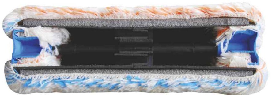
Cross-section of FASADA roller with foam backing
